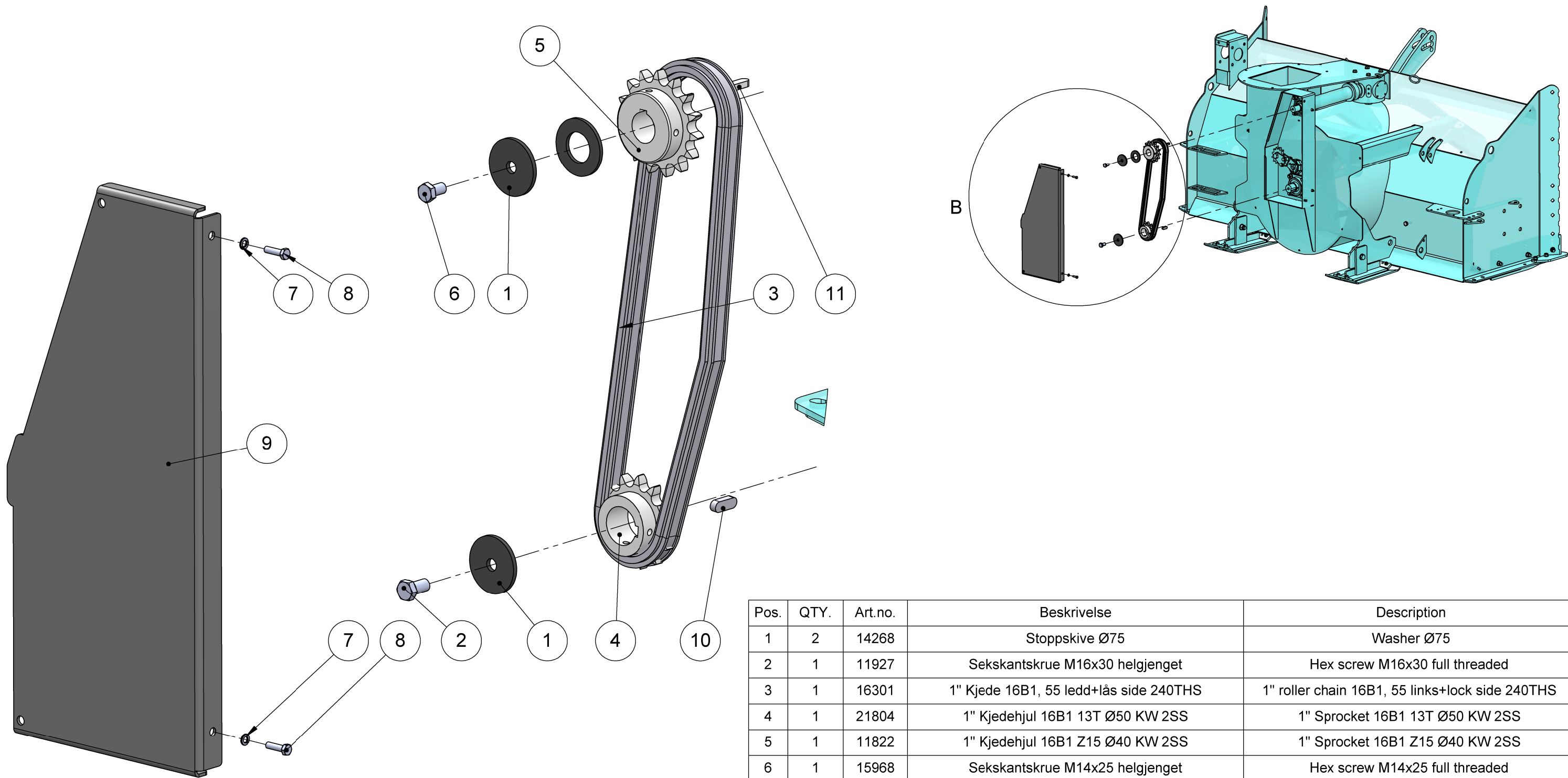
DETAIL B
